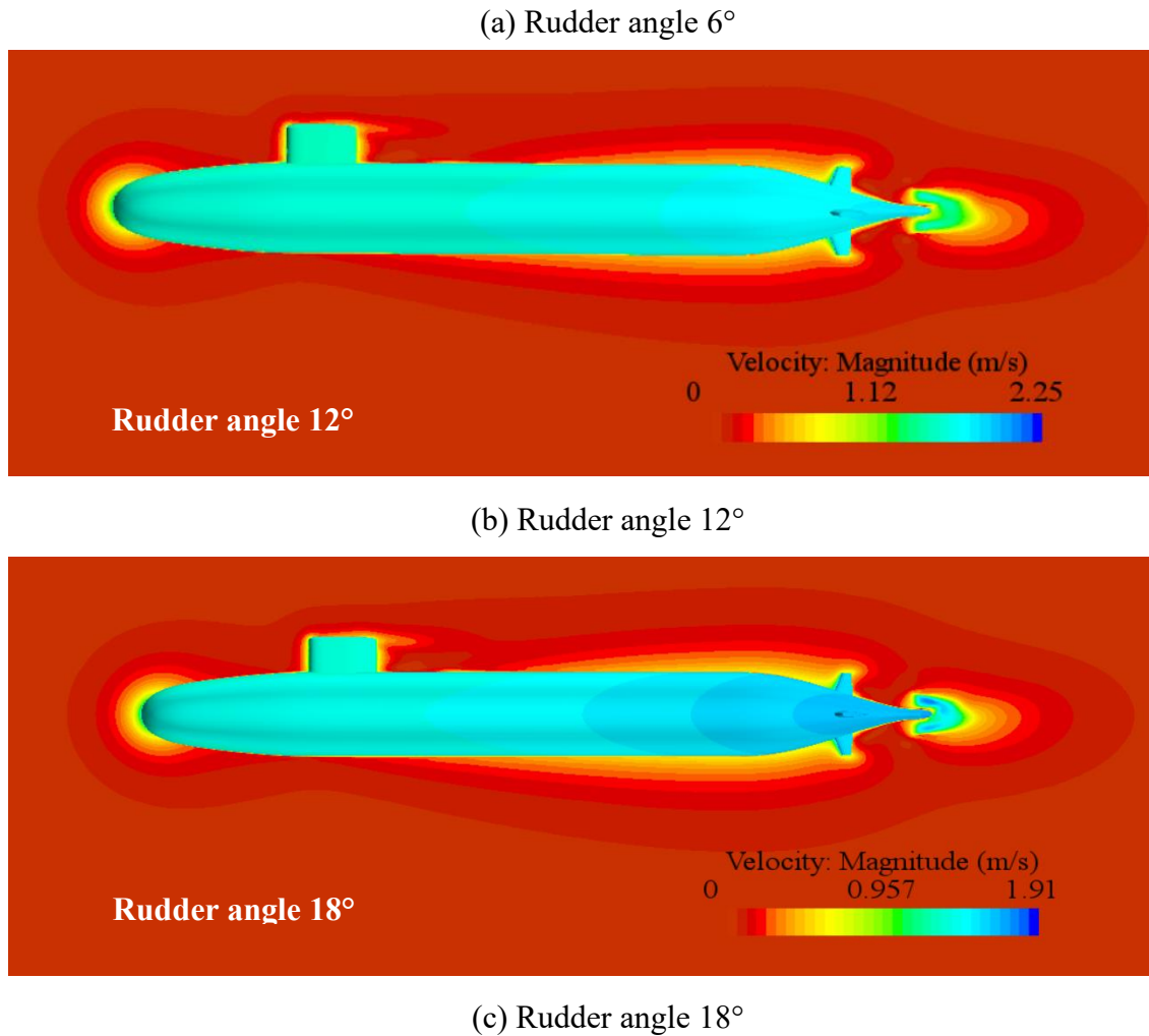
Figure. 18. Velocity nephogram corresponding to different rudder angles (middle longitudinal section)
