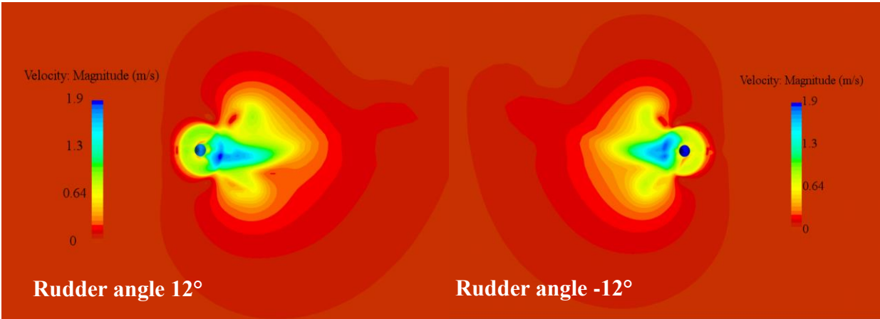
(b) Rudder angle -12^\circ/12^\circ
