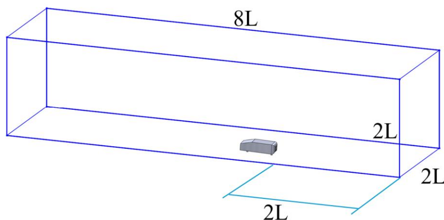
Figure. 3. Modeling of the Ahmed experiment.
